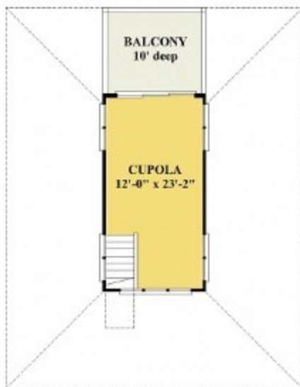
THIRD FLOOR PLAN 254 HEATED SQUARE FEET
